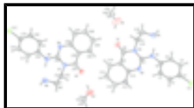
Fig. 1. View of the molecular structure of (I), showing the atom labelling scheme and with displacement ellipsoids drawn at the 50% probability level.
