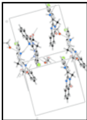
Fig. 2. A partial view of the crystal packing of (I), showing the formation of N—H...N, O—H...O and N—H...O hydrogen-bonds (dashed lines).
